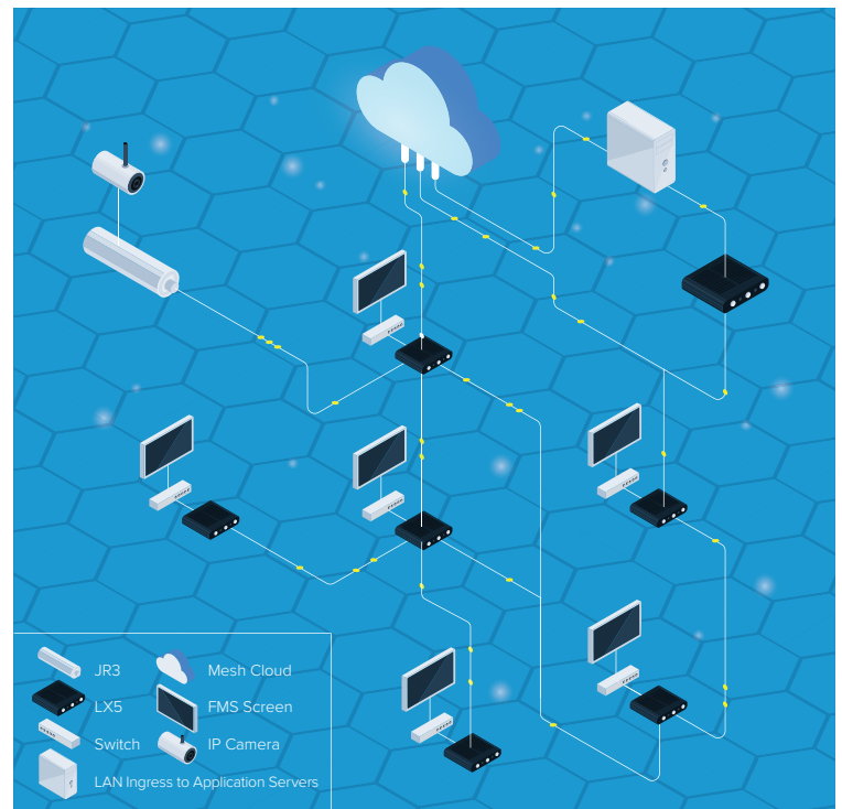
JR3 BreadCrumbs are optimal for edge applications such as supporting a video surveillance camera in a busy intersection or processing plant.
